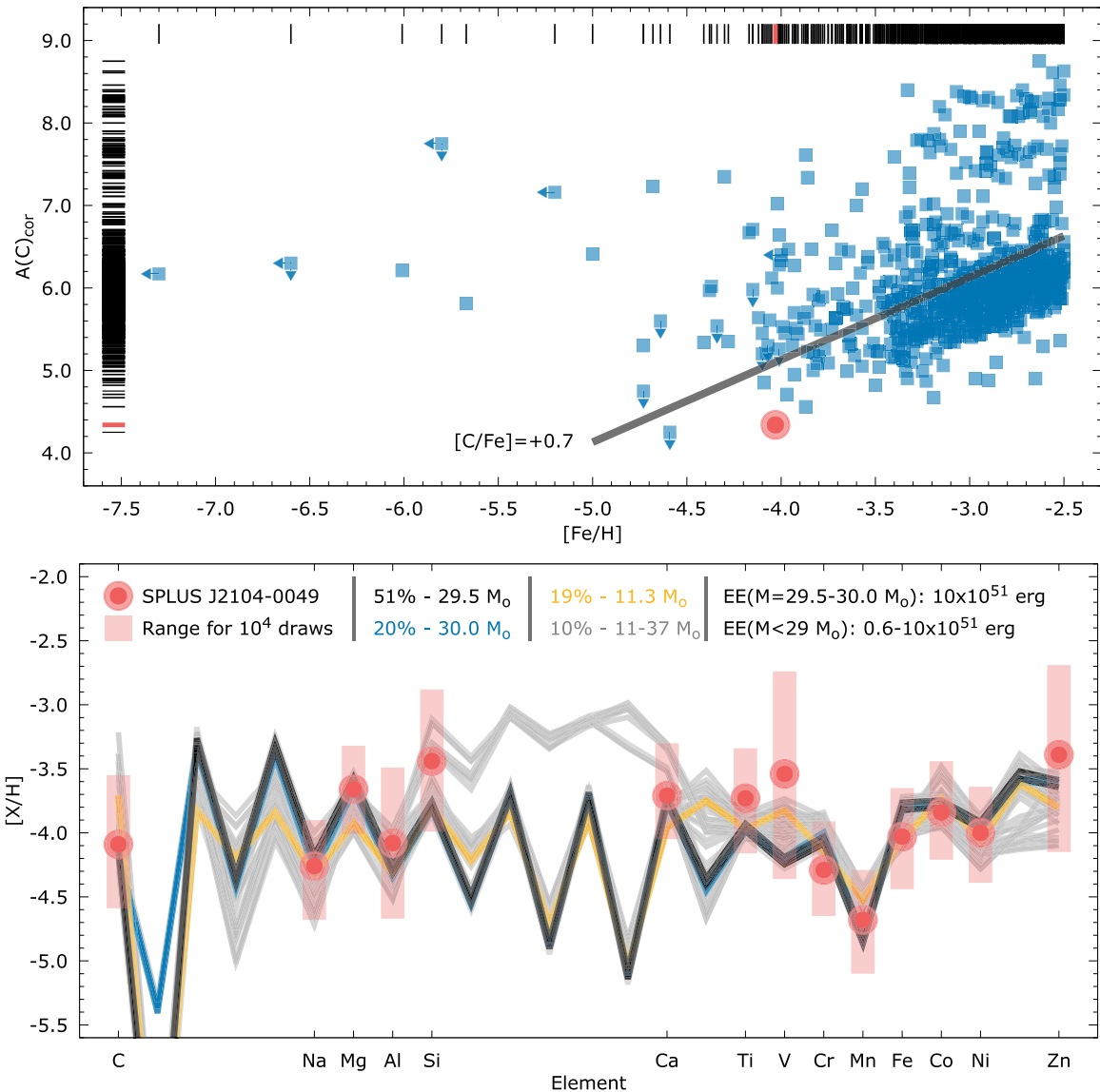
Figure 3. Upper panel: carbon abundances— A(C) —as a function of the metallicity— [Fe/H] —for SPLUS J2104–0049 (filled circle) and the literature compilations JINAbase (Abohaima & Frebel 2018) and SAGA (Suda et al. 2008) (filled squares). The solid line represents the current criteria for CEMP stars ( [C/Fe] = +0.7 ). Upper limits are only shown for [Fe/H] \leq -4.0 . Stripe-density profiles are also shown, with the values for SPLUS J2104–0049 highlighted. The upper panel is also available as a Bokeh-generated interactive figure. Hovering the mouse over any point will reveal the underlying data including the name, atmospheric parameters, carbon abundances, upper limit flags, and source. Other functionalities are available via the buttons at the top of the interactive figure. Hovering the mouse over each will reveal its functionality, i.e., panning, zooming, reset. The underlying data set is also available in machine-readable format via the figure data file link. A bigger version that will be updated as more data become available is available at http://vmlplacco.github.io/files/acfeh.html . Lower panel: best model fits for SPLUS J2104–0049. The solid lines show the theoretical predictions from the Heger & Woosley (2010) znuc2012.s4 models, color coded by mass and occurrence fraction within the 10^4 simulations. The explosion energies (EEs) are also listed. The solid circles are the measured abundances for SPLUS J2104–0049, and the shaded areas mark the range of simulated abundances.
