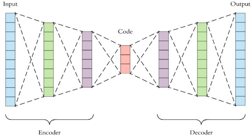
Fig. 2. Autoencoder architecture
