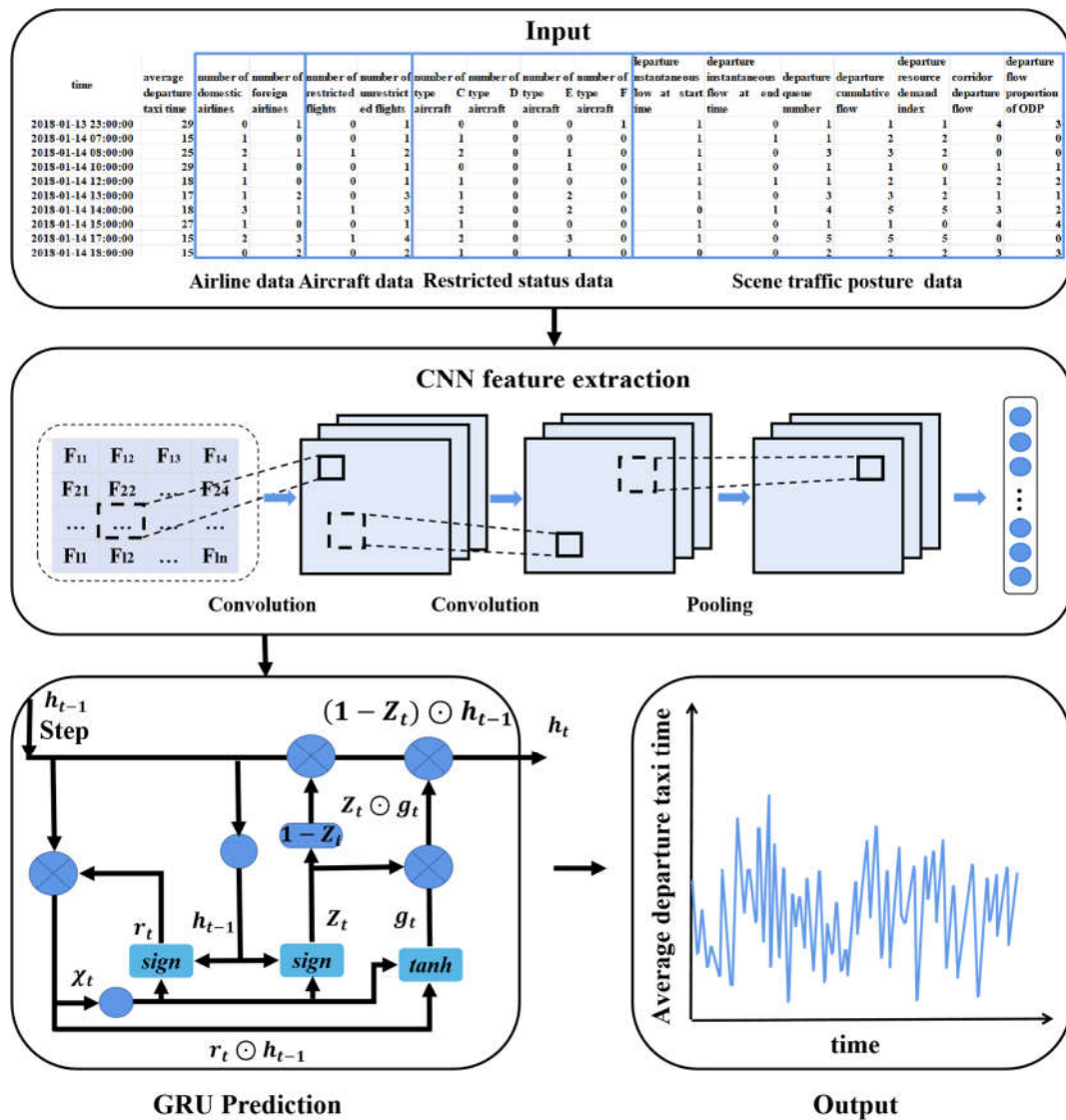
Figure 5. CNN-GRU-based departure taxiing time prediction model.
