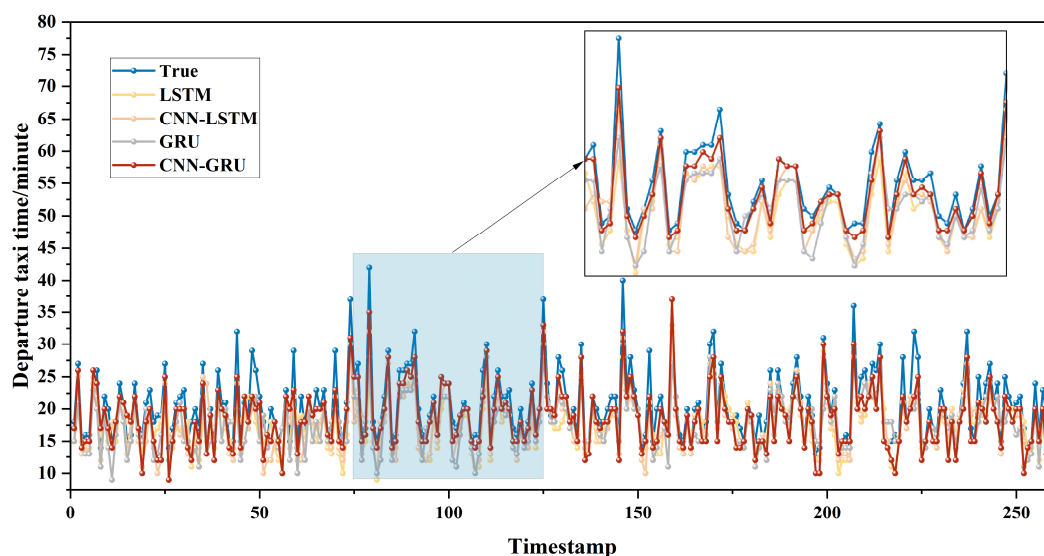
Figure 6. Prediction results of different models.
