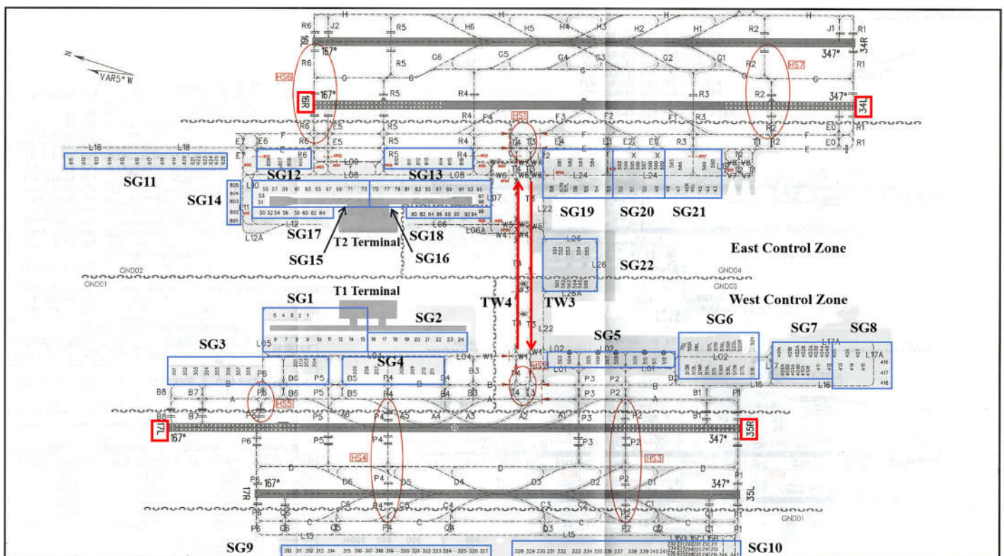
Figure 1. Layout of Pudong International Airport.
