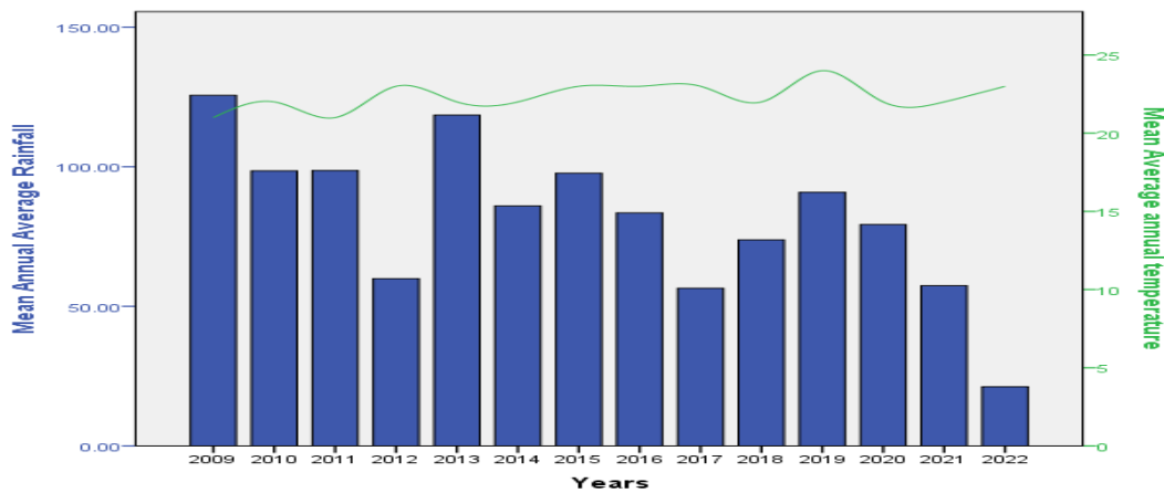
Fig. 4. Annual rainfall and annual temperature
