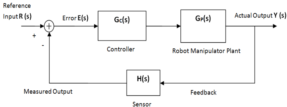
Fig. 1. A block diagram of a closed-loop control system
