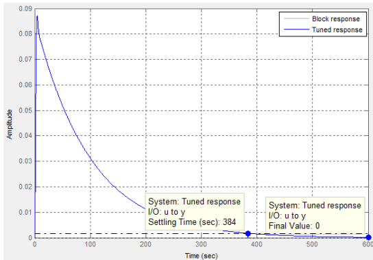
Fig. 4a. Step disturbance rejection of A
