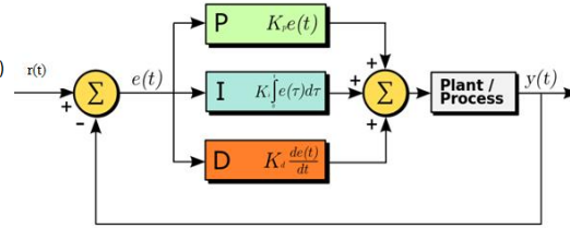
Fig. 2b. PID controller in a closed-loop system
