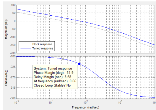
Fig. 6b. Bode plot for an unstable system
