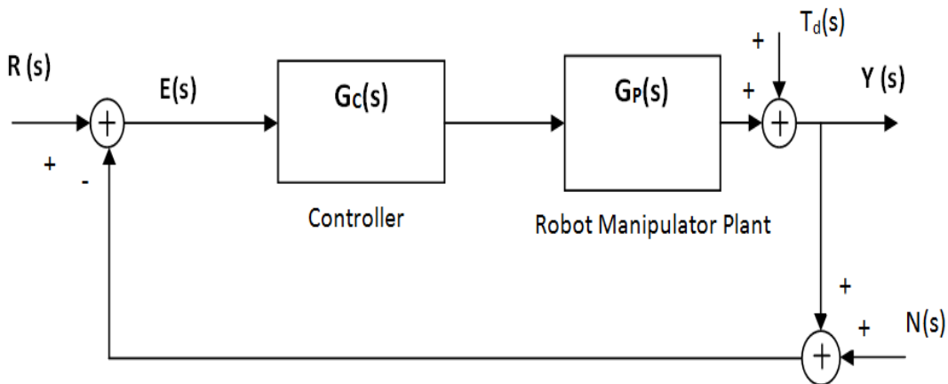
Fig. 3. Control system with disturbance and noise inputs in real environment
