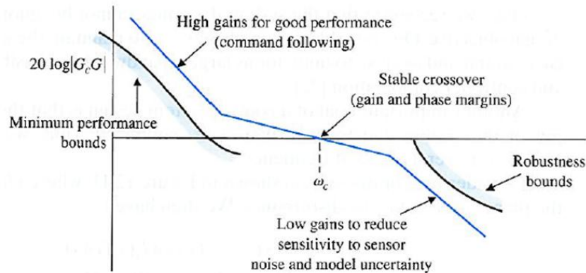
Fig. 5. Demonstration of system behavior on Bode plot [18]
