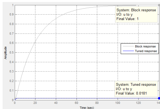
Fig. 4c. Step disturbance rejection of C
