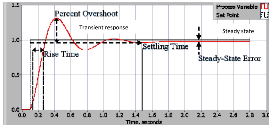
Fig. 7. Step reference tracking response of a PID closed-loop control system
