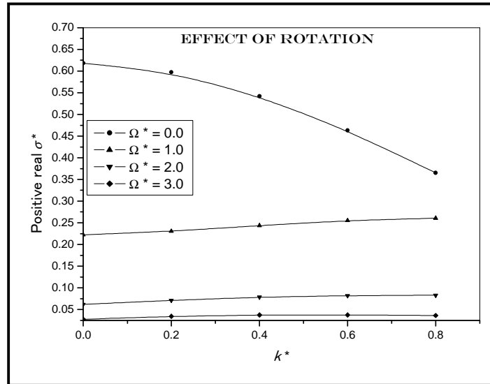
Fig. 2. The growth rate is plotted against the non-dimensional wave number k^* with variation in the normalized rotational effect \Omega^* = 0.0, 1.0, 2.0, 3.0 the value \lambda^* = \nu^* = \nu_c^* = \eta^* = V^* = 1 and the value of \mathcal{L}_T^* = 0.0 and \mathcal{L}_\rho^* = 0.5
