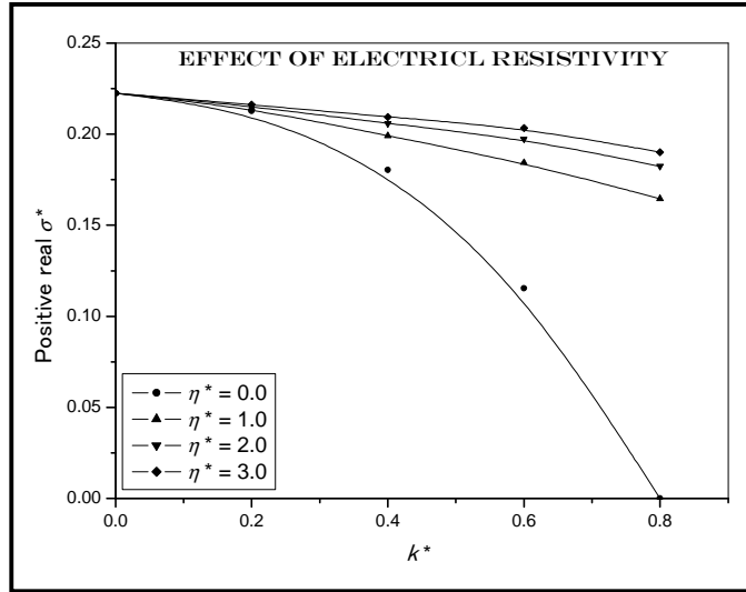
Fig. 3. The growth rate is plotted against the non-dimensional wave number k^* with variation in the normalized resistivity effects \eta^* = 0.0, 1.0, 2.0, 3.0 the value \lambda^* = \nu^* = \nu_c^* = V^* = \Omega^* = 1 and the value of \mathcal{L}_T^* = 0.5 and \mathcal{L}_\rho^* = 0.0
