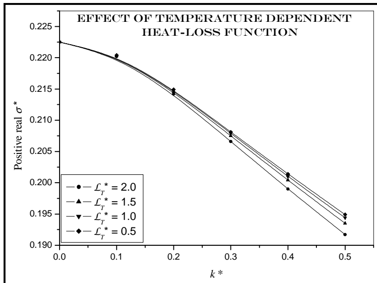
Fig. 6. The growth rate is plotted against the non-dimensional wave number k^* with variation in the normalized temperature dependent hit loss function effects the value \mathcal{L}_T^* = 0.5, 1.0, 1.5, 2.0 the value V^* = \nu_c^* = \nu^* = \lambda^* = \eta^* = \Omega^* = 1 and the value of \mathcal{L}_\rho^* = 0.0
