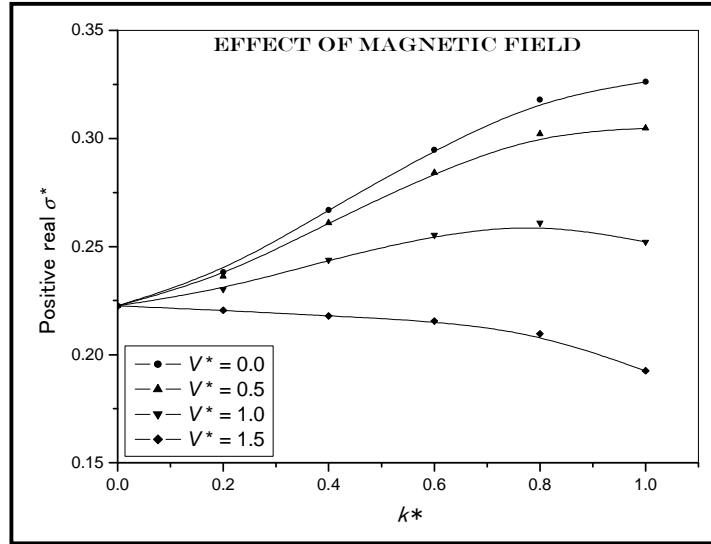
Fig. 1. The growth rate is plotted against the non-dimensional wave number k^* with variation in the normalized magnetic field V^* = 0.0, 0.5, 1.0, 1.5 the value \lambda^* = \nu^* = \nu_c^* = \eta^* = \Omega^* = 1 and the value of \mathcal{L}_T^* = 0.0 and \mathcal{L}_\rho^* = 0.5
