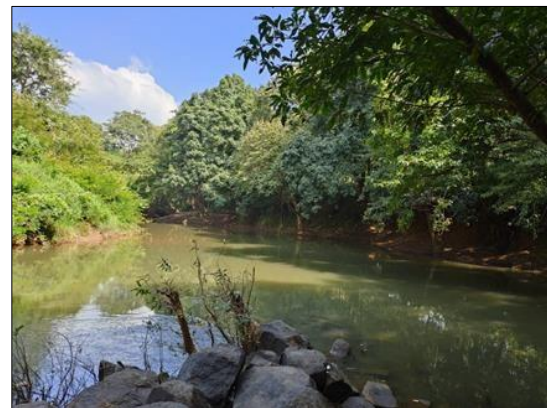
Fig. 11. 4 th order stream of sub watershed
