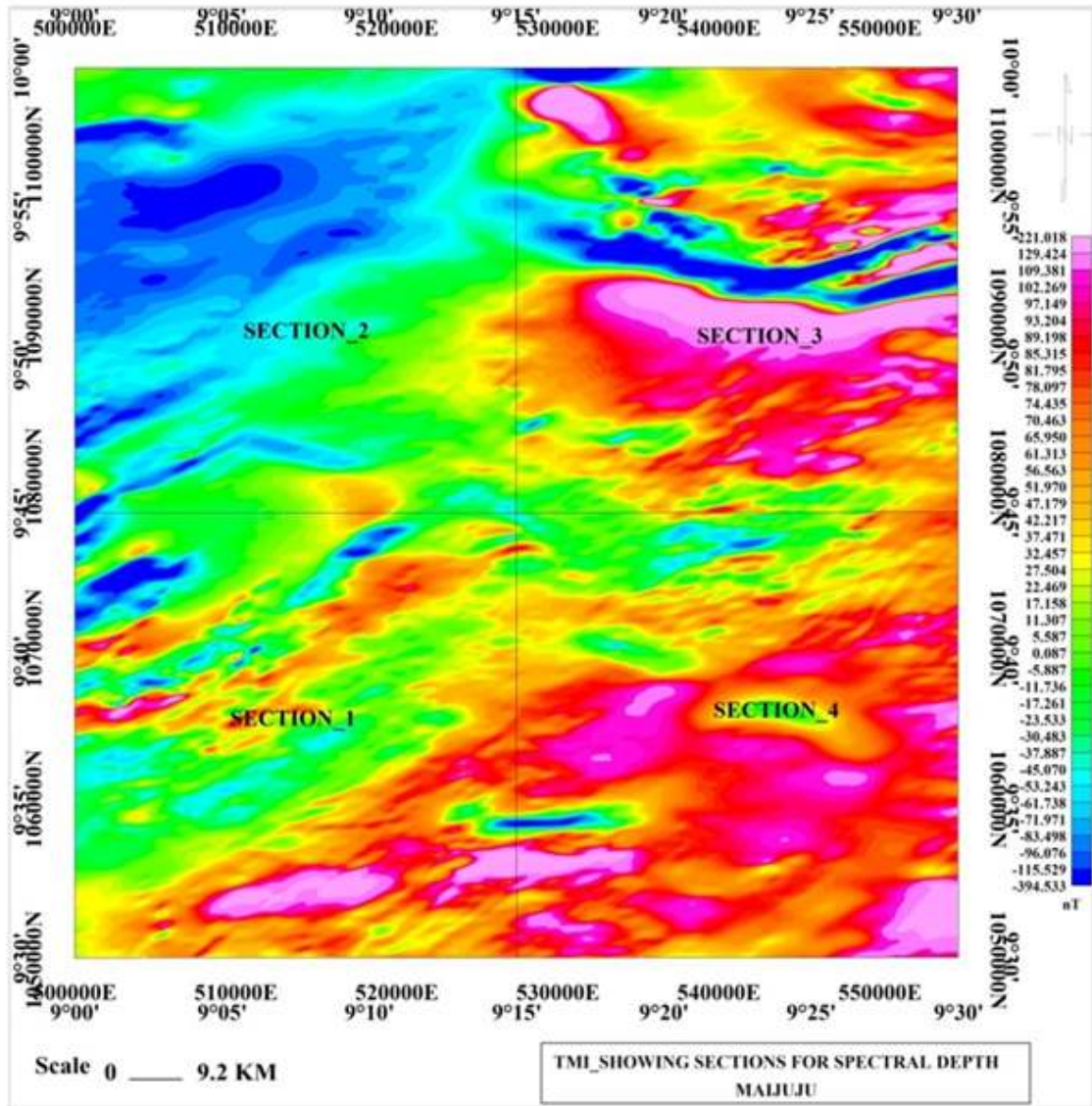
Fig. 7. TMI showing sections selected for spectral depth
