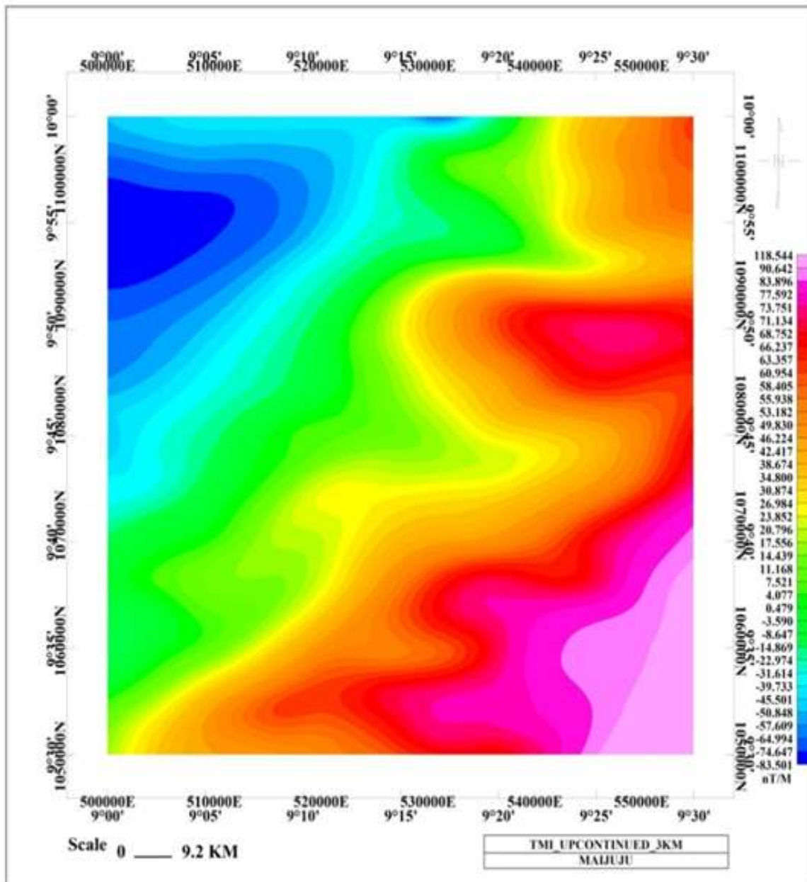
Fig. 6. TMI data continued upward to 3 km elevation
