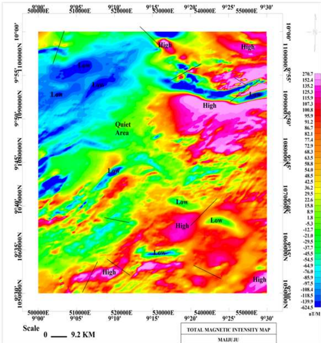
Fig. 2. Total magnetic intensity (TMI) map of Maijuju sheet 169, with lines representing dislocations
