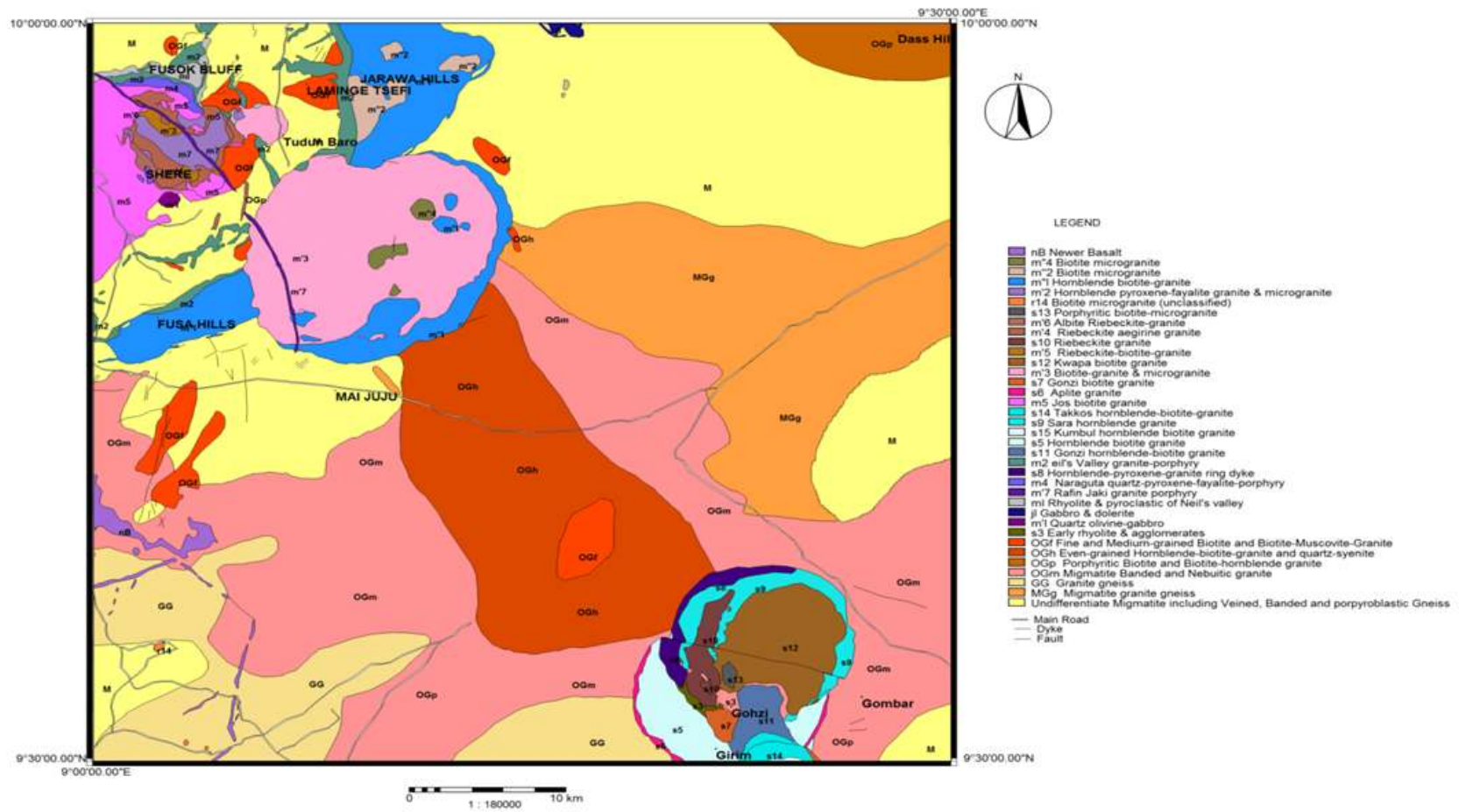
Fig. 1. Digitised geology map of Maijuju sheet 169. (After geological survey of Nigeria, 1962)
