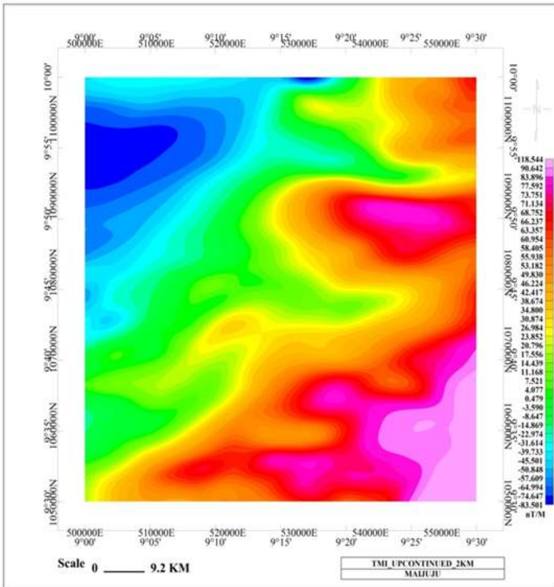
Fig. 5. TMI data continued upward to 2 km elevation
