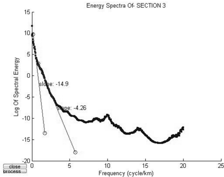
Fig. 10. Plot of log of spectral energy against frequency for section 3
