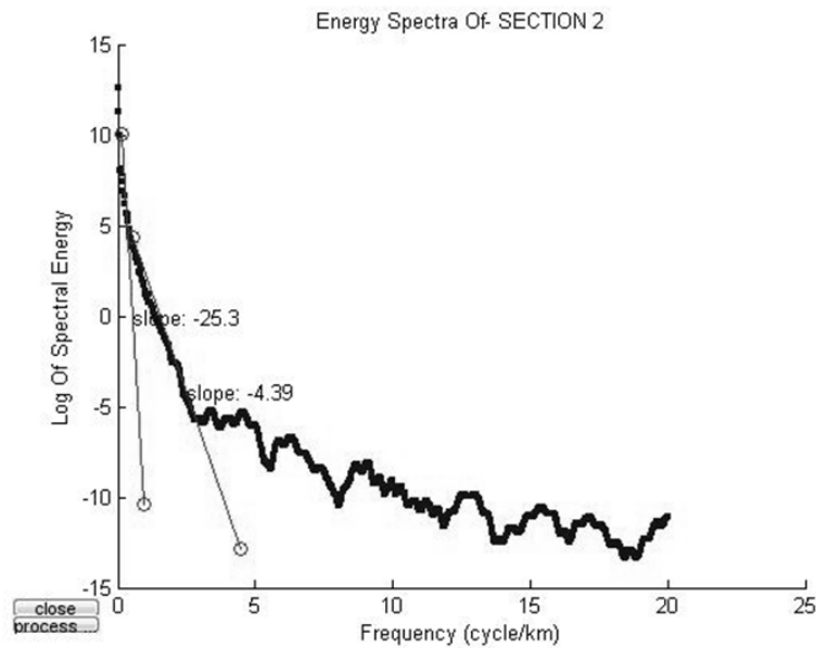
Fig. 9. Plot of log of spectral energy against frequency for section 2
