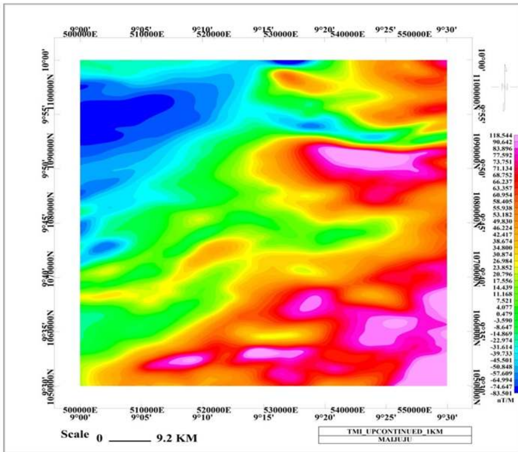
Fig. 4. TMI data continued upward to 1 km elevation
