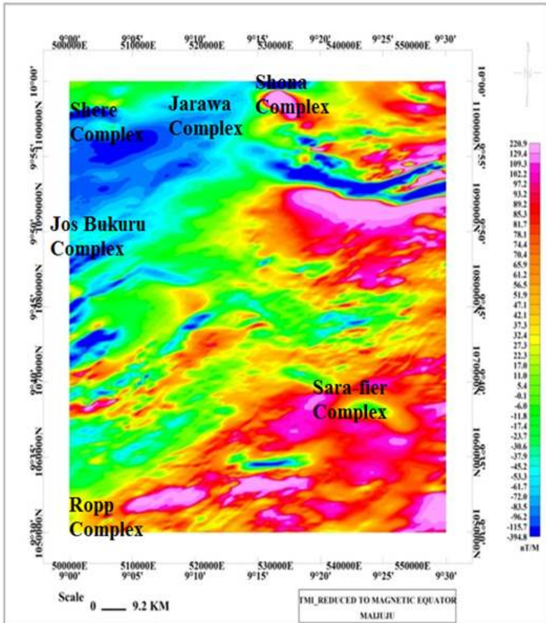
Fig. 3. Total magnetic intensity reduced to equator (TMI-RTE) map
